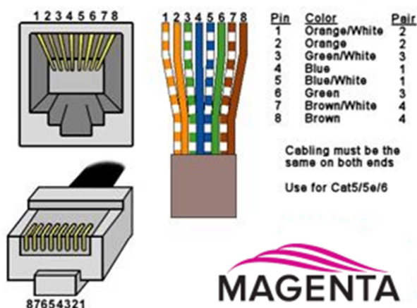
Figure 3: T568B CAT5 Specification
