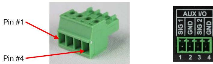
Figure 5: 4-pin Phoenix Connector Pinout
