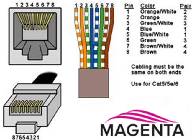
Figure 8: T568B CAT5
