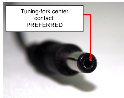
Figure 7: Tuning-fork Connector
