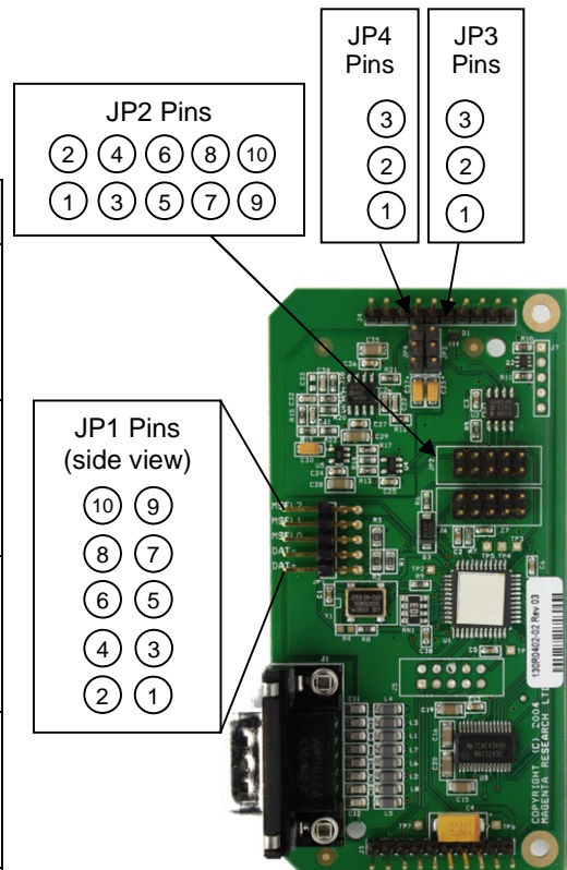
Figure 12: Receiver (232) Module Board
