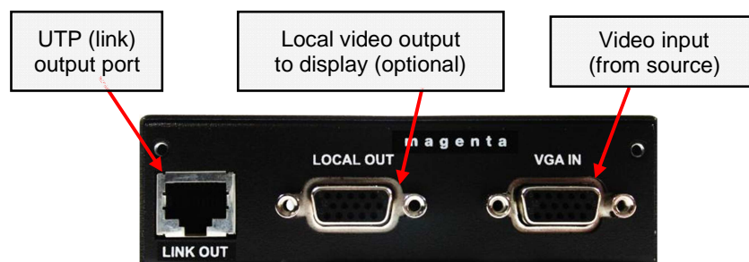
Figure 2: Rear Panel Interfaces
