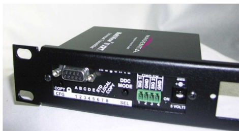
Figure 16: XRTx with 1U Rack-mount Plate
