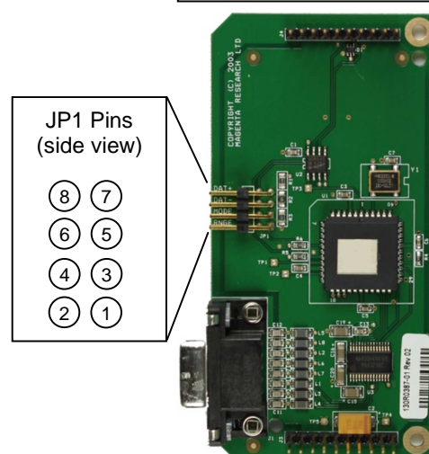
Figure 11: Transmitter (232) Module Board
