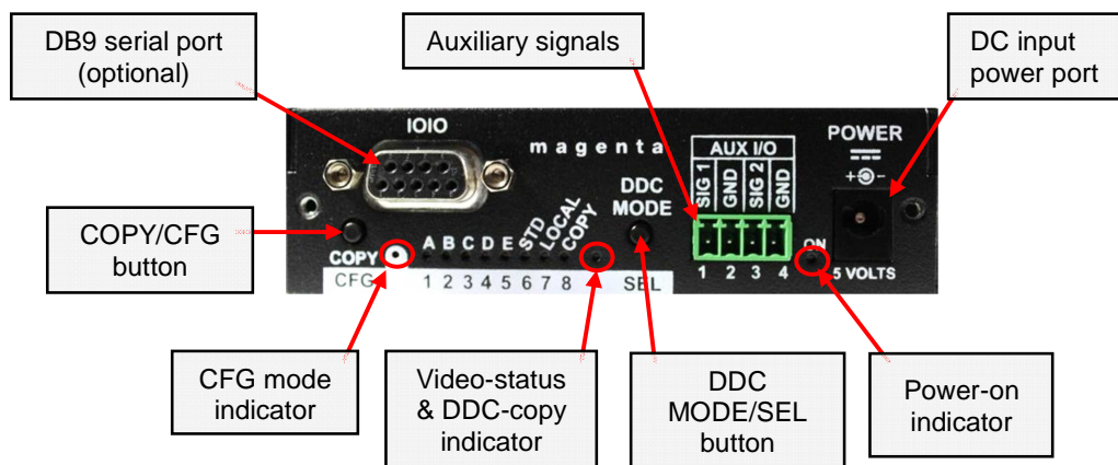
Figure 1: Front Panel Interfaces
