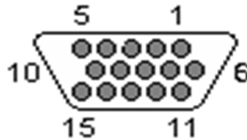
Figure 10: HD-15 Female Connector
