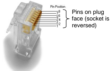
Figure 9: Typical RJ-45 Plug
