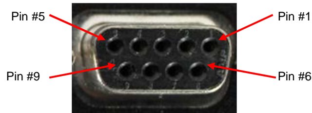
Figure 4: DB9-F Serial Port
