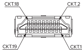
HDMI Type A Pin Assignment
