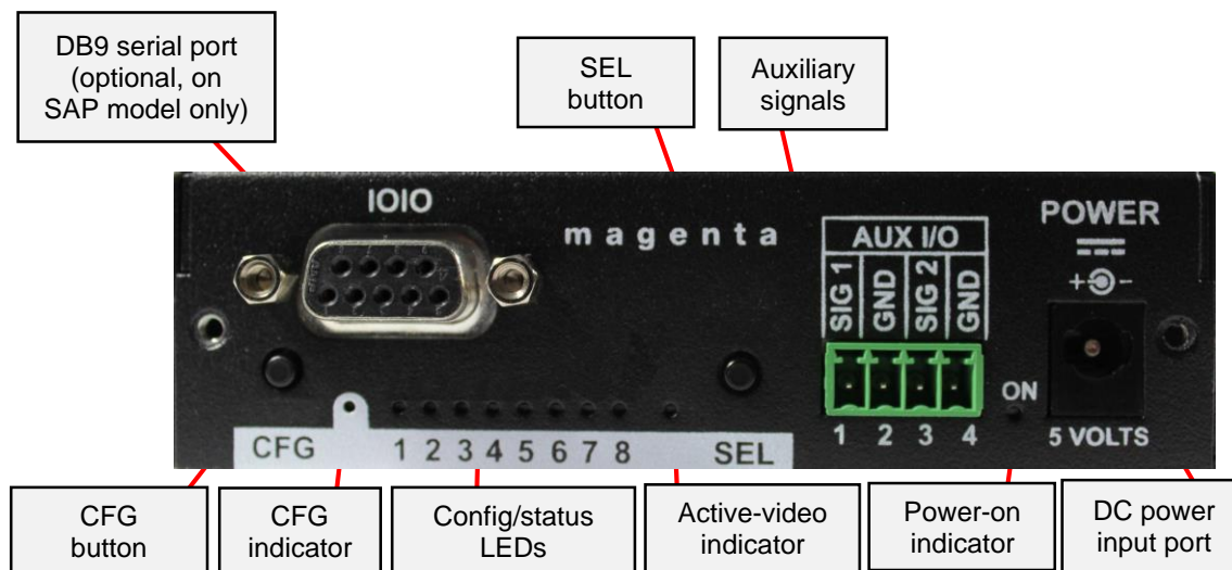
Figure 1: MVII-DVI-Tx Front Panel Interfaces
