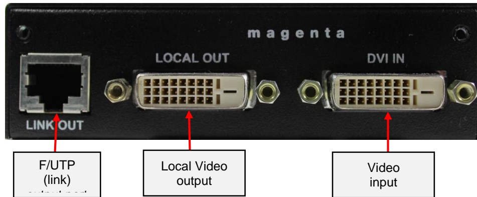
Figure 2: MVII-DVI-Tx Rear Panel Interfaces
