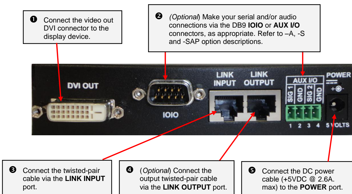
Figure 4: MVII-DVI-Rx-1K Receiver connections
