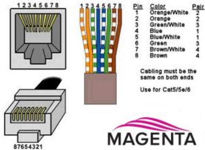
Figure 8: T568B Category Cable Wiring Standard
